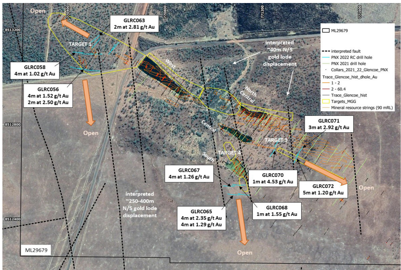
Figure 7 Glencoe November 2022 RC drilling, with interpreted faults shown as dashed lines.
