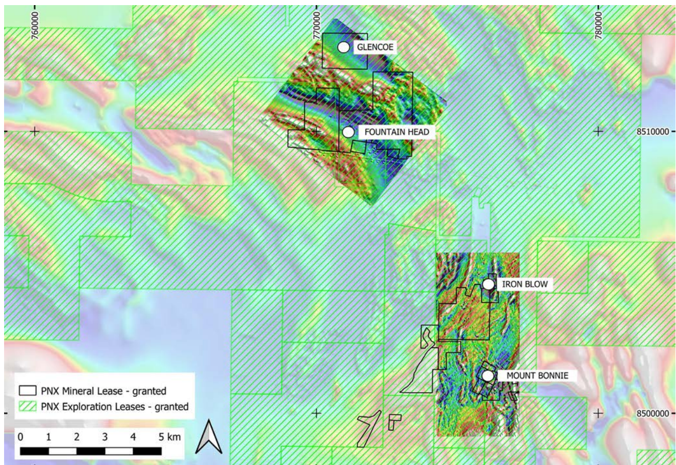
Figure 5 New magnetic imagery from recent drone survey over the Glencoe and Fountain Head gold, and Mt Bonnie and Iron Blow zinc-gold-silver deposits. Background image: regional Total Magnetic Intensity.
