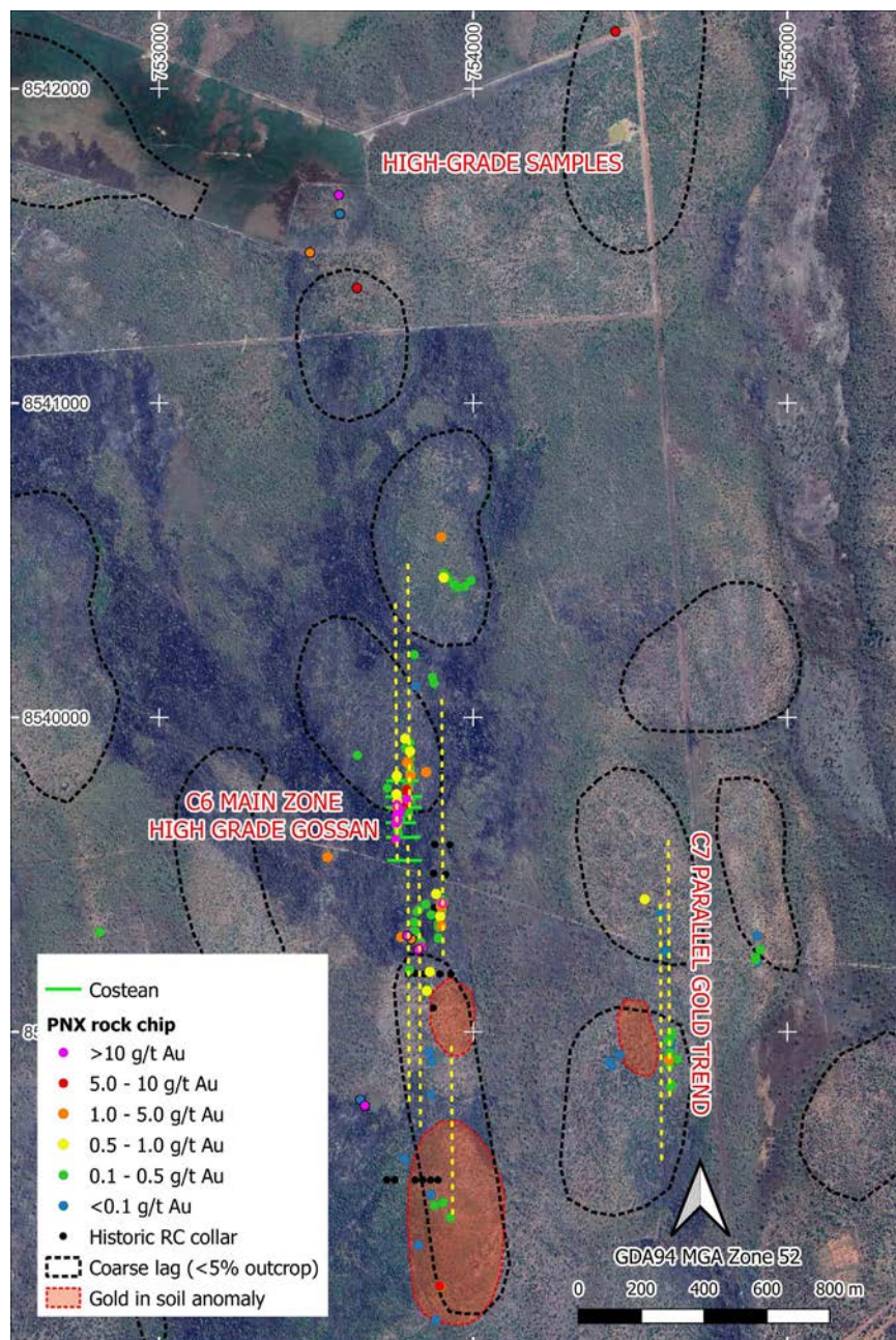
Figure 3 PNX rock chips and costeans (green lines), historic drilling and limited historic soil anomalies. Yellow dashed lines represent interpreted gold trends.
