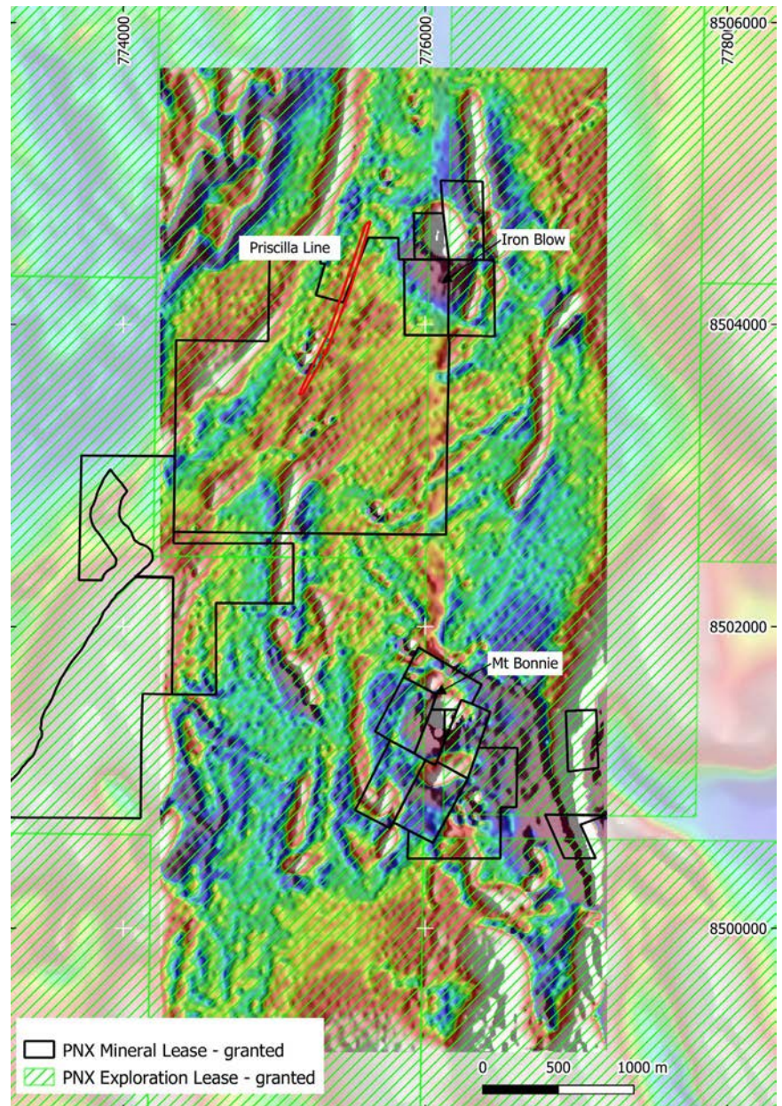
Figure 8 Coloured Total Magnetic Intensity draped over first vertical derivative for Hayes Creek drone survey. Areas highlighted (white rings) refer to discrete magnetic-highs of interest.
