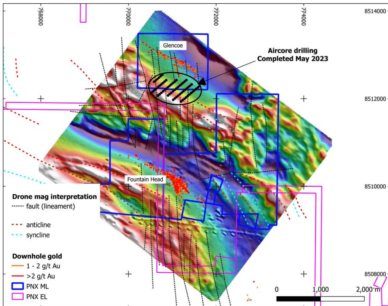
Figure 6 Location of aircore drilling between Glencoe and Fountain Head over drone magnetic Total Magnetic Intensity.
