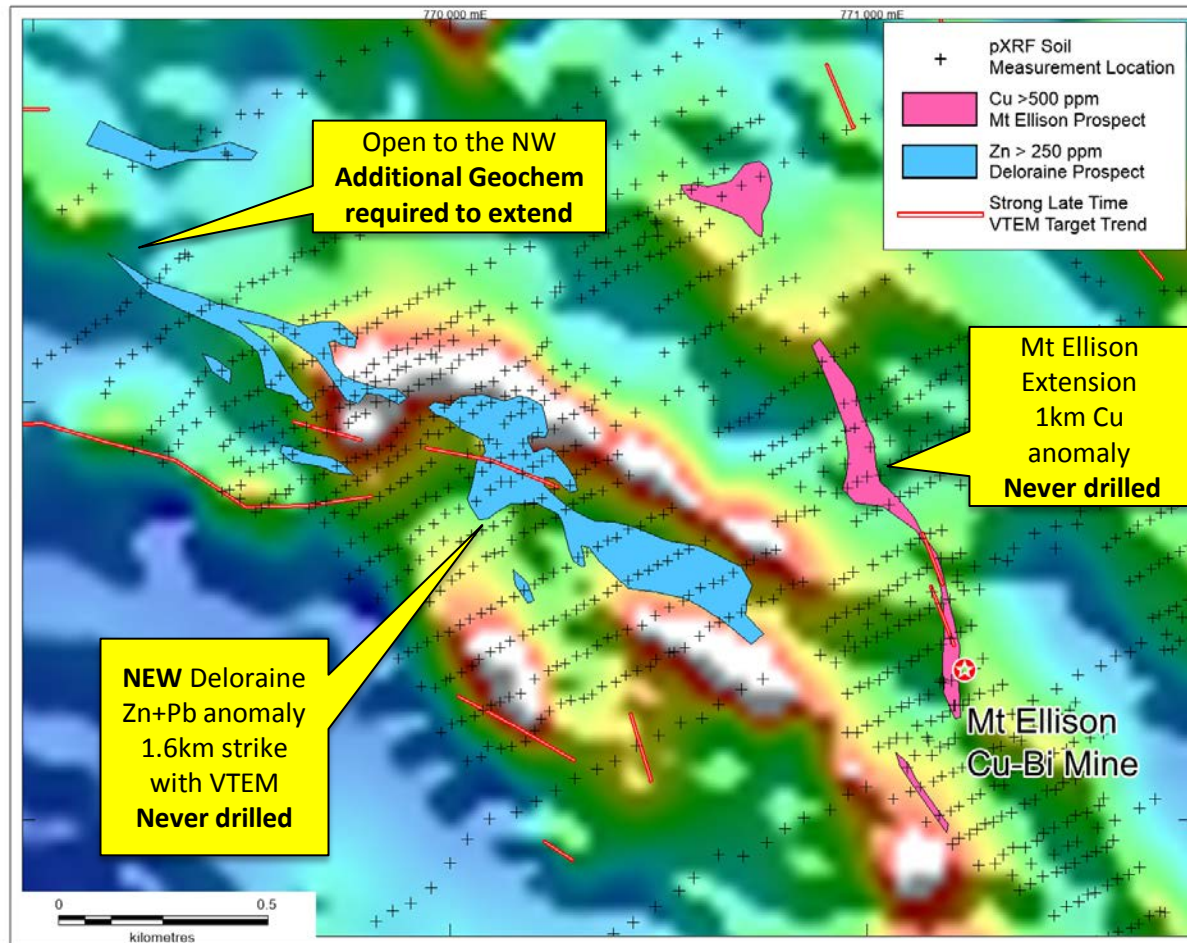
VTEM image dBdt Z38
